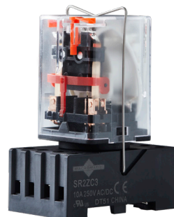
Retainer on GR120A2w Relay and SR2ZC3 Socket
